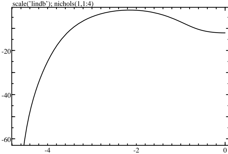
Figure 10.20 scale('lindb'); nichols(1,1:4)
