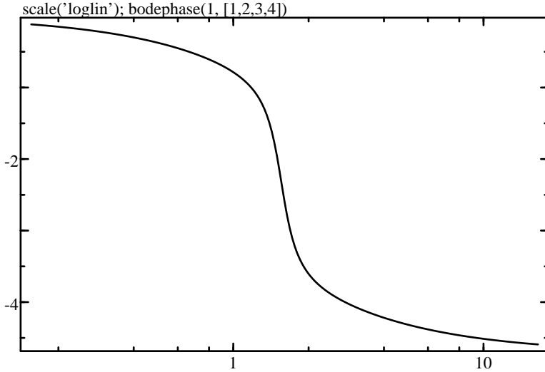
Figure 10.10 scale('loglin'); bodephase(1, [1,2,3,4])
