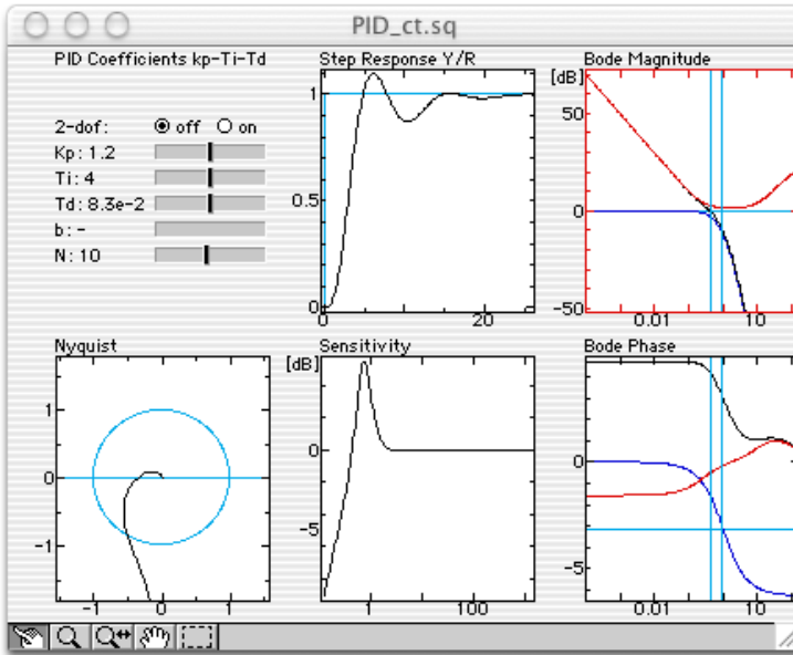
Figure 4.1 PID_ct.sq
