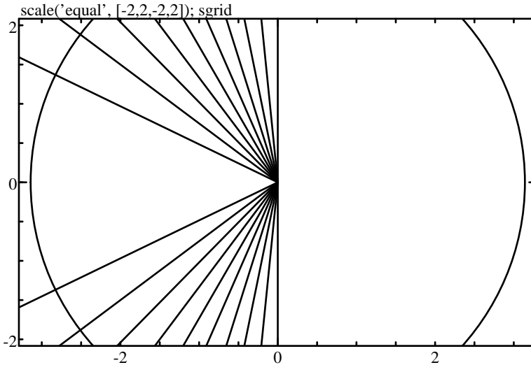
Figure 10.23 Result of sgrid when the whole grid is displayed.
