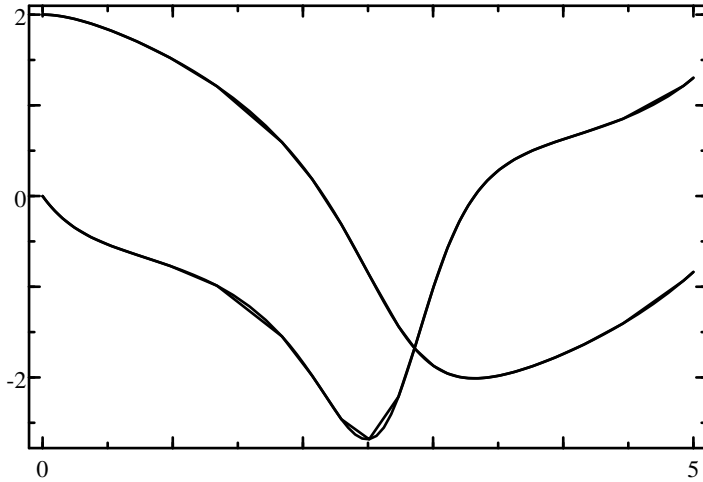
Figure 10.2 Van der Pol equation with Refine set to 1 and 4
