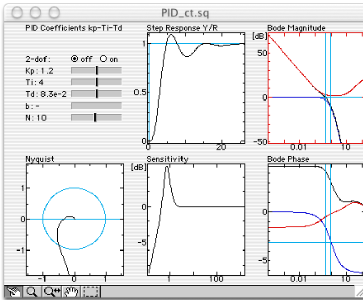
Figure 4.1 PID_ct.sq
